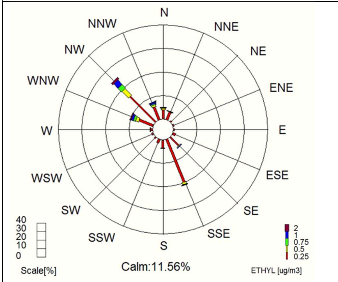
Pollution Rose for EthylBenzene ( \mu\text{g}/\text{m}^3 ) 01/06/2022 00:00 – 30/11/2022 24:00 Station O.L. Volos AVG: 15min
