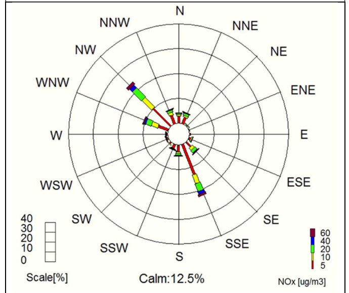
Pollution Rose for NO x ( \mu\text{g}/\text{m}^3 ) 01/06/2022 00:00 – 30/11/2022 24:00 Station O.L. Volos AVG: 5min
