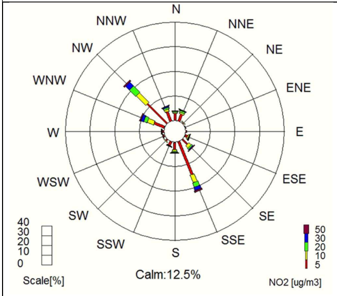
Pollution Rose for NO 2 ( \mu\text{g}/\text{m}^3 ) 01/06/2022 00:00 – 30/11/2022 24:00 Station O.L. Volos AVG: 5min
